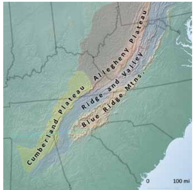
Figure 1. Geographic regions of the Appalachian physiographic division.
